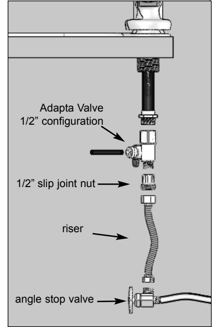
B. Water supply line with Adapta Valve in 1/2" configuration
