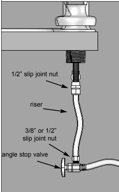
Water supply line before installation
