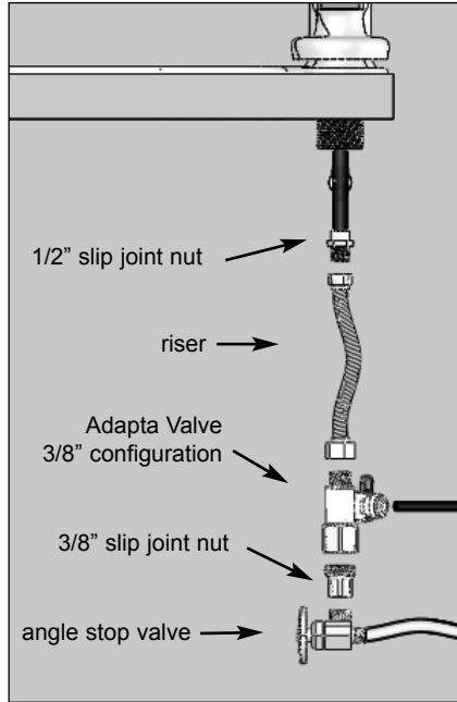
A. Water supply line with Adapta Valve in 3/8" configuration
